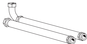
1 x flexible pipe with bend (WN2) 1 x flexible pipe (WN3) (Dimensions, flexible pipes DN25, G1¼") 4 x gaskets
