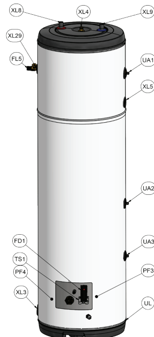
NIBE MEGACOIL 160, 200, 300 and 400
