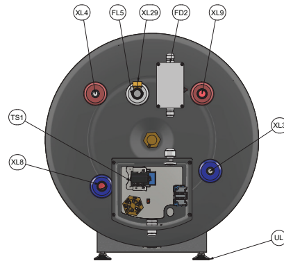
NIBE MEGACOIL 160, 200, 300 and 400
