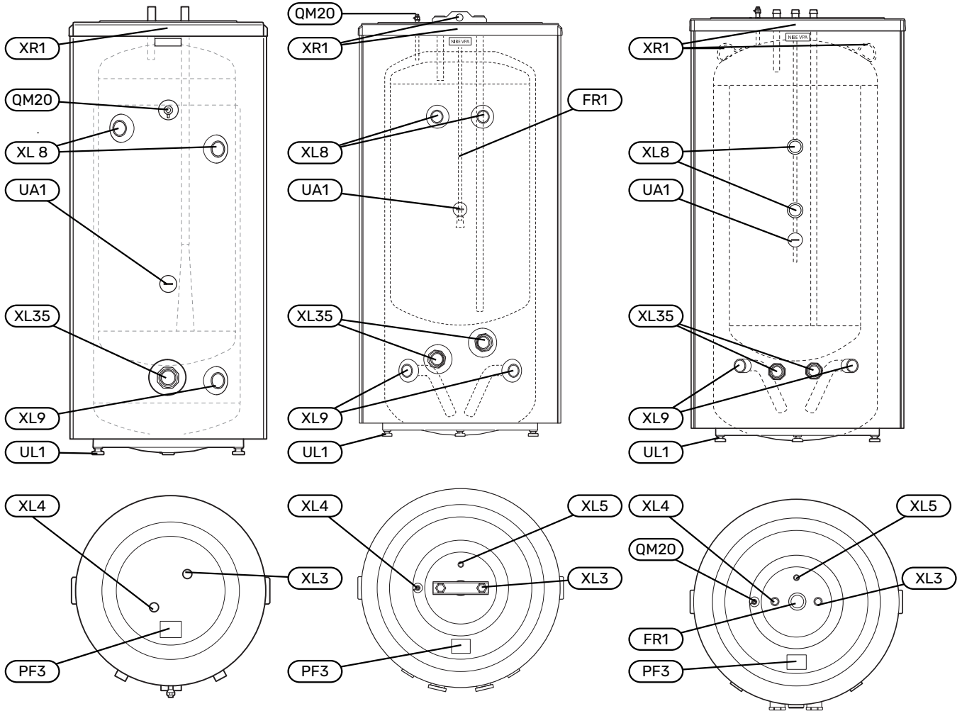
VPA 200/70 Copper
