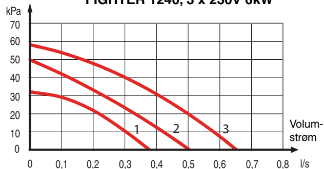
FIGHTER 1240, 3 x 230V 6kW
