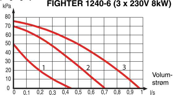
FIGHTER 1240-6 (3 x 230V 8kW)
