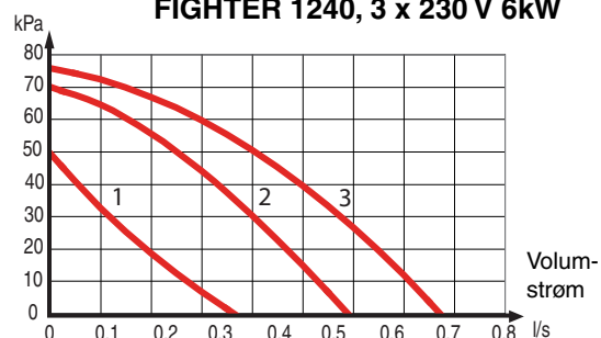
FIGHTER 1240, 3 x 230 V 6kW
