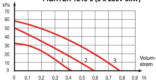
FIGHTER 1240-6 (3 x 230V 8kW)
